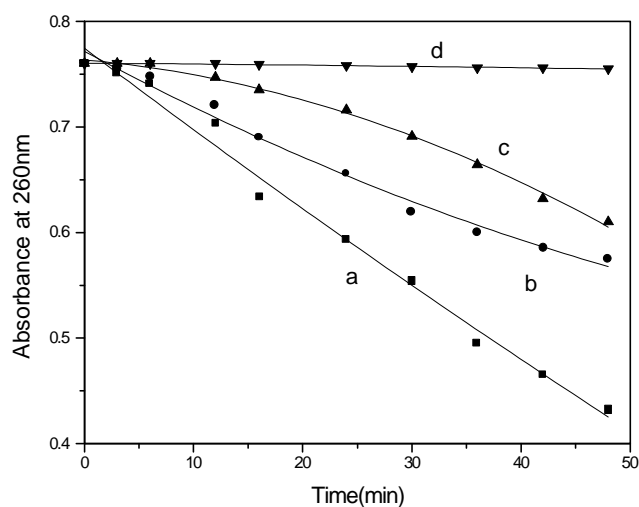
Figure 1. Effect of caffeic acid on the photooxidation of adenosine by PDS [adenosine] = 5.00 \times 10^{-5} \text{ mol dm}^{-3} , [PDS] = 4.00 \times 10^{-4} \text{ mol dm}^{-3} , [caffeic acid] = (a) 0.0, (b) 5.00 \times 10^{-6} \text{ mol dm}^{-3} , (c) 1.00 \times 10^{-5} \text{ mol dm}^{-3} , (d) 5.00 \times 10^{-5} \text{ mol dm}^{-3} . Light intensity = 1.01 \times 10^{15} \text{ quanta s}^{-1} .
